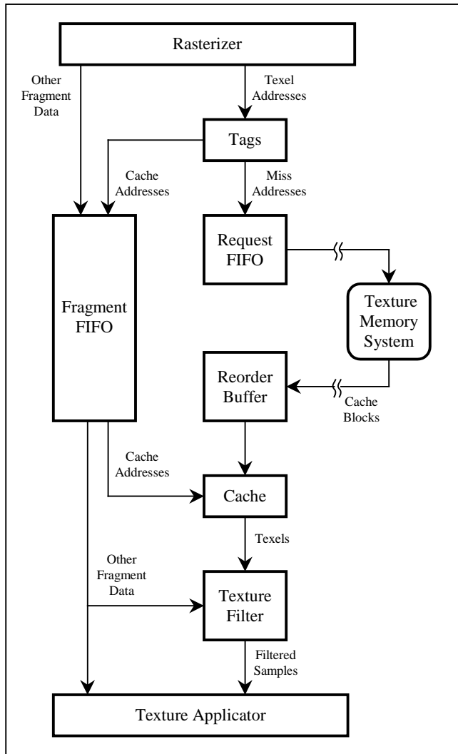
Figure 2: A Texture Prefetching Architecture.
