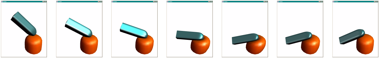
Figure 5: Simulation of a kinematically constrained rigid object contacting a deformable object. This is a difficult problem because the contact boundary conditions keep changing during the motion. ARTDEFO solves such a sequence of problems quickly by combining precomputed system responses using a rank update procedure. It is possible to perform multiple solves each frame in order to guarantee unilateral contact constraints are satisfied.
